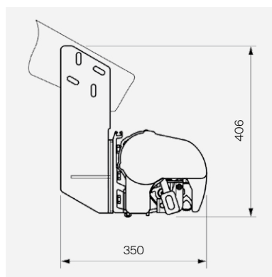
Balkmontering vertikalt
