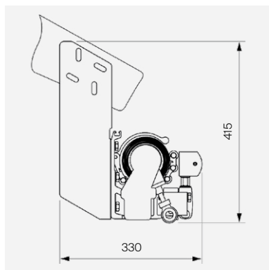
Balkmontering vertikalt
