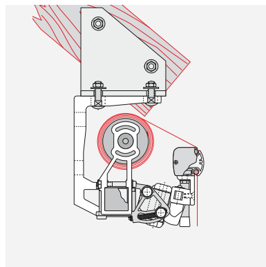
Balkmontering vertikalt
