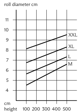
RECOMMENDED ROLL DIAMETER
