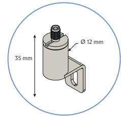
Gripper for wall mounting
