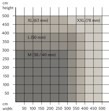
MOTOR - TUBE DIMENSION FOR FABRIC WEIGHT UP TO 250 G/M 2
